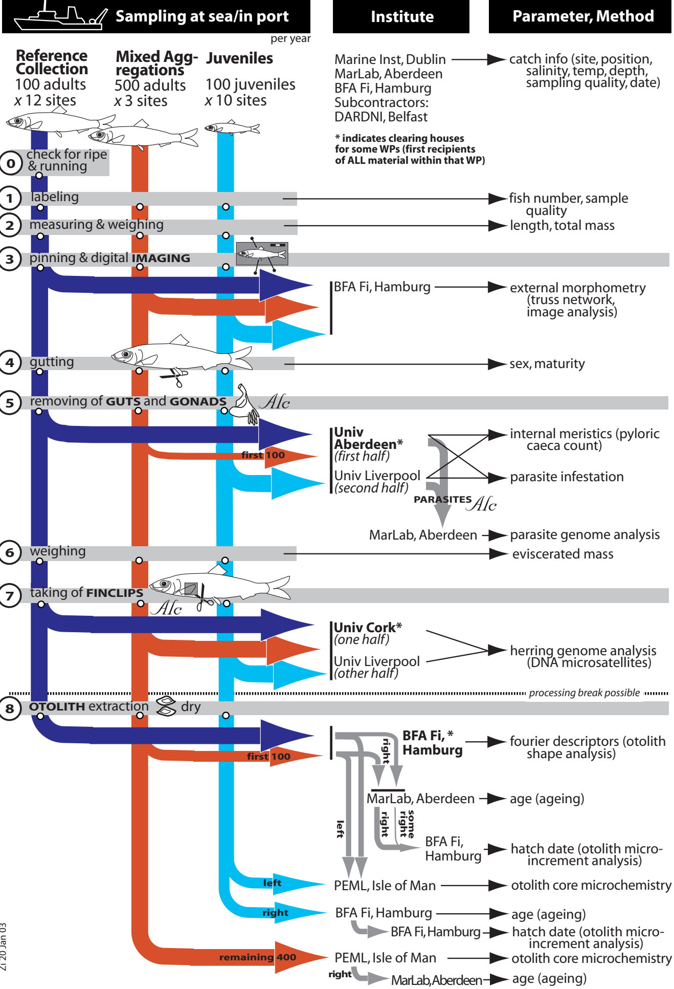
EU-Project WestHer : sample flow scheme
